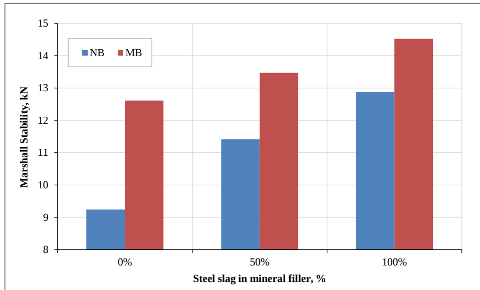
Figure 6. the Marshall stability of mixtures
