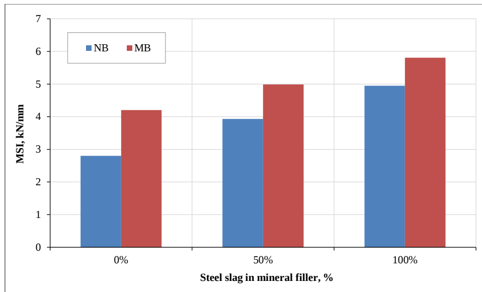
Figure 8. Marshall Stiffness Index (MSI) of Mixtures
