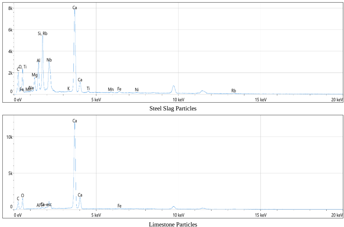
Figure 12. The EDX analysis results
