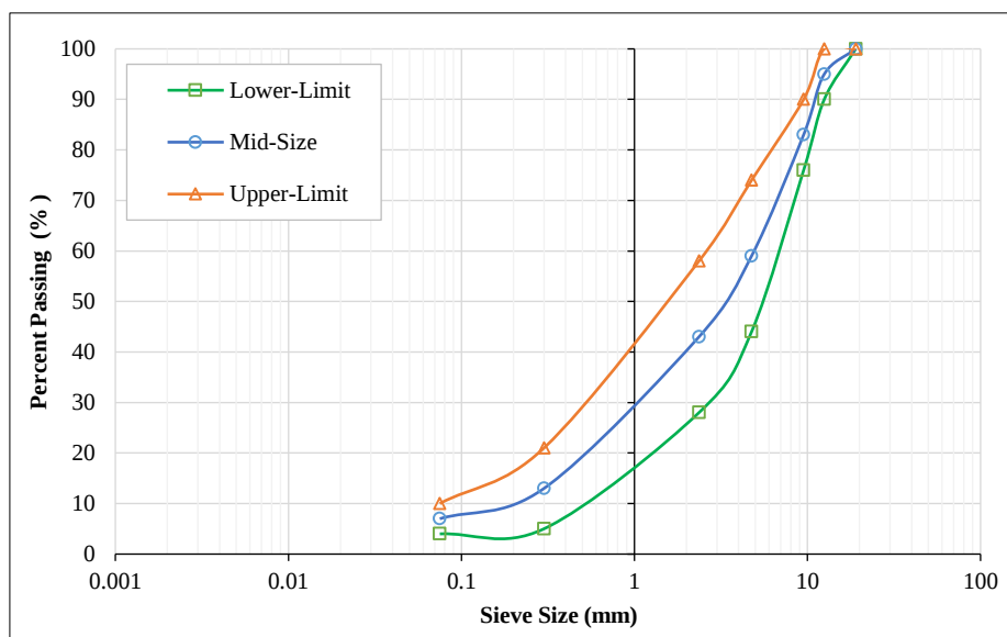
Figure 2. Aggregate particle gradation against the limits for surface course
