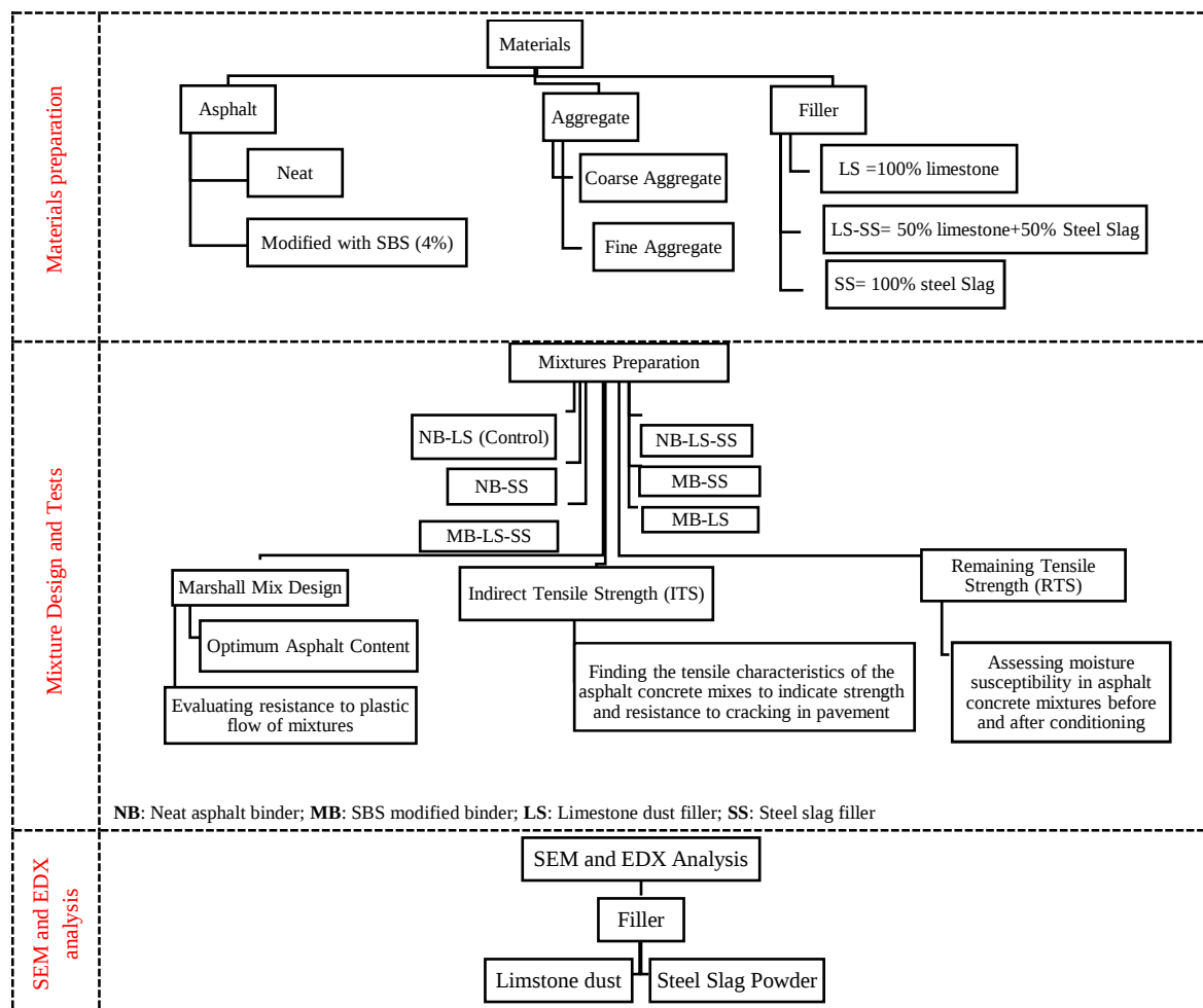
Figure 1. The flow chart of experimental study
