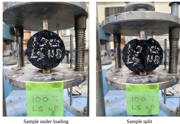
Figure 4. The indirect tensile test
