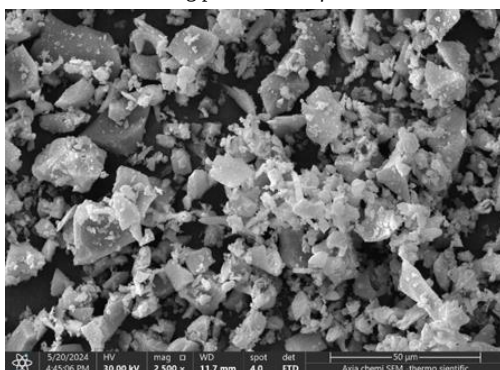
Steel slag particle at 50 \mu\text{m} scale
