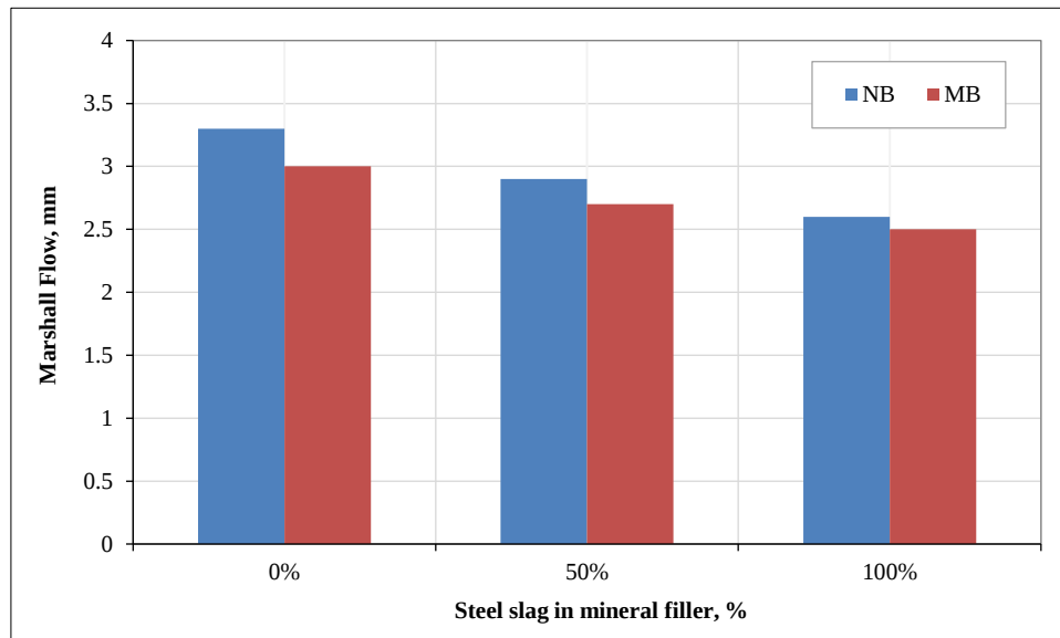
Figure 7. Marshall Flow of mixtures
