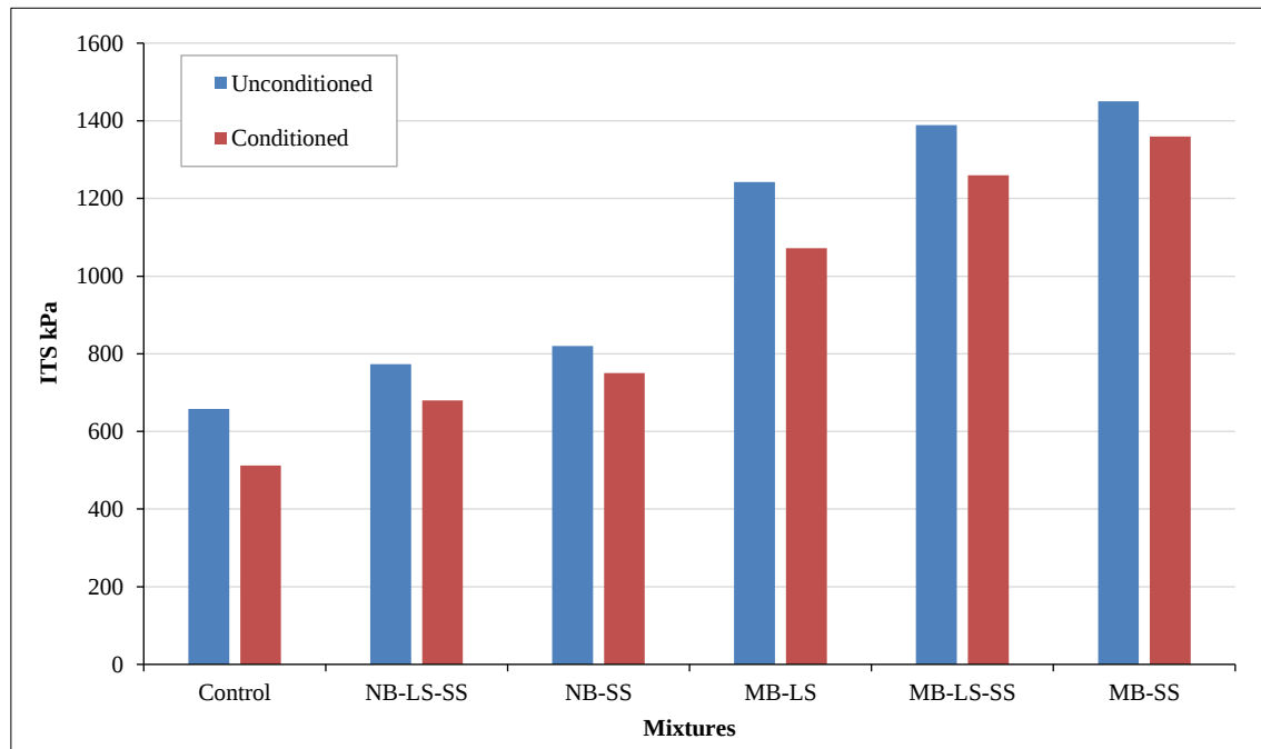
Figure 9. Indirect Tensile Strength (ITS) test results
