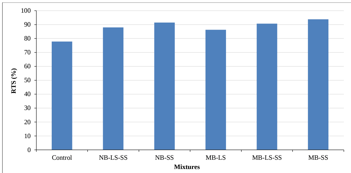
Figure 10. The Remaining Tensile Ratio results for the different types of mixtures
