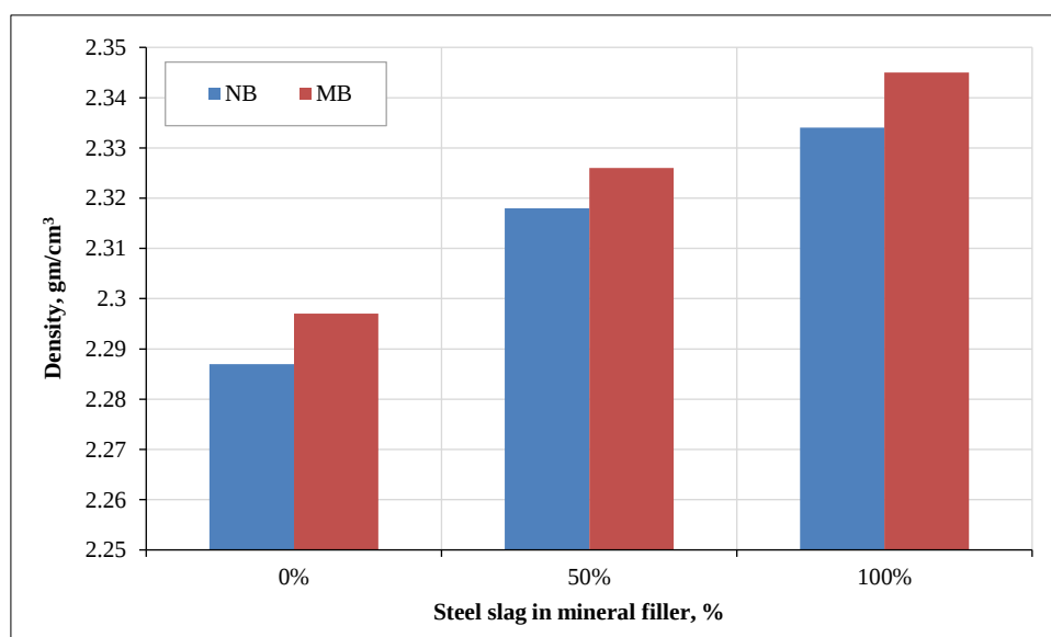
Figure 5. The density of mixtures
