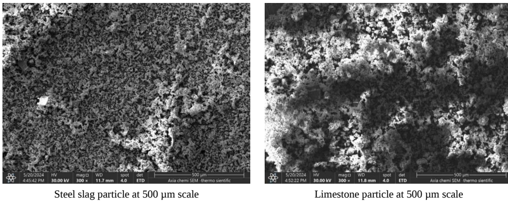
Figure 11. SEM images for the microscopic characteristics of SS and LS particles
