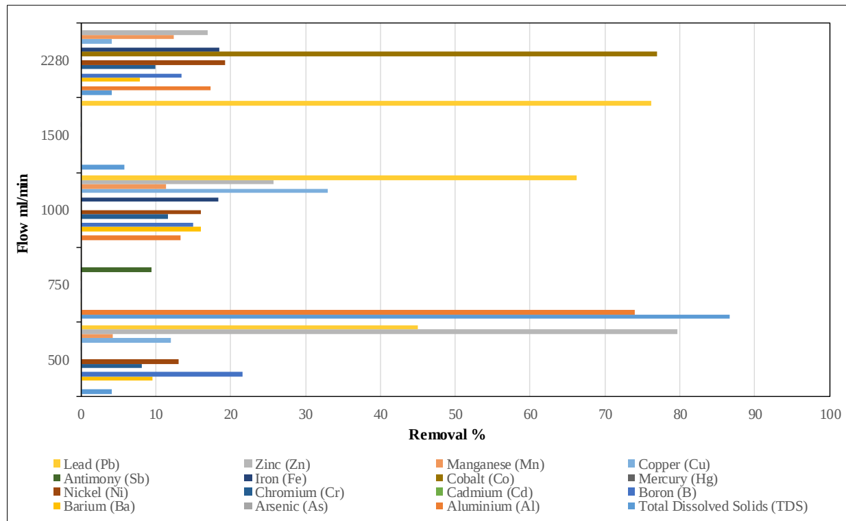
Figure 8. Removal of selected parameters from high-strength wastewater under 16 kHz at different flow rates
