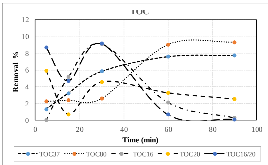
Figure 6. TOC removal under different ultrasound operating conditions
