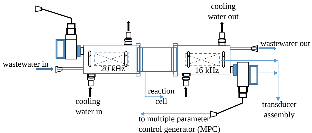
Figure 2. Schematic of the dual-frequency ultrasound flow-through reactor
