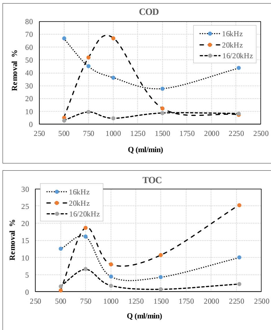
Figure 4. Medium-strength wastewater sonication in the flow-through ultrasound reactor
