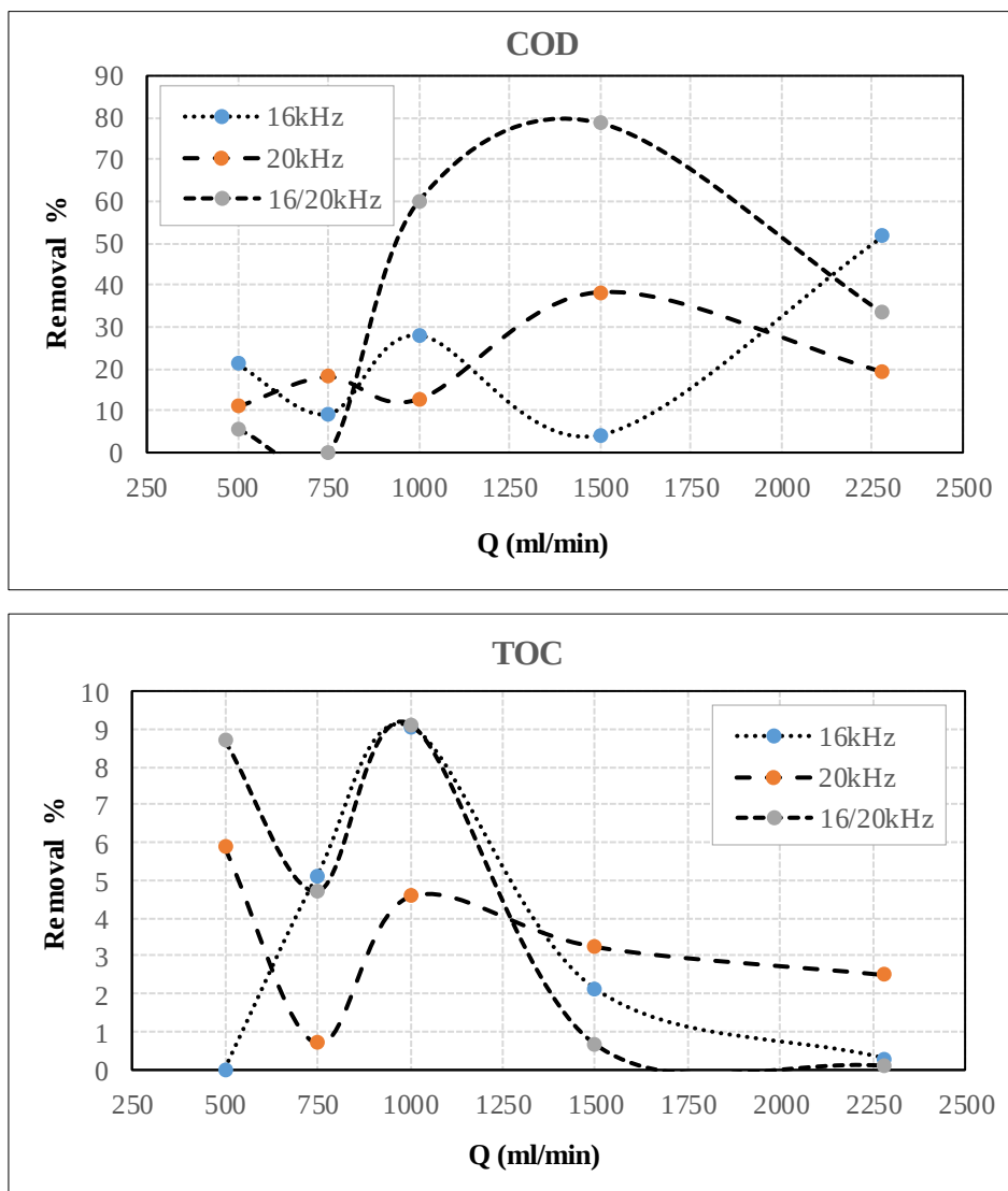
Figure 5. Low-strength wastewater sonication in the flow-through ultrasound reactor
