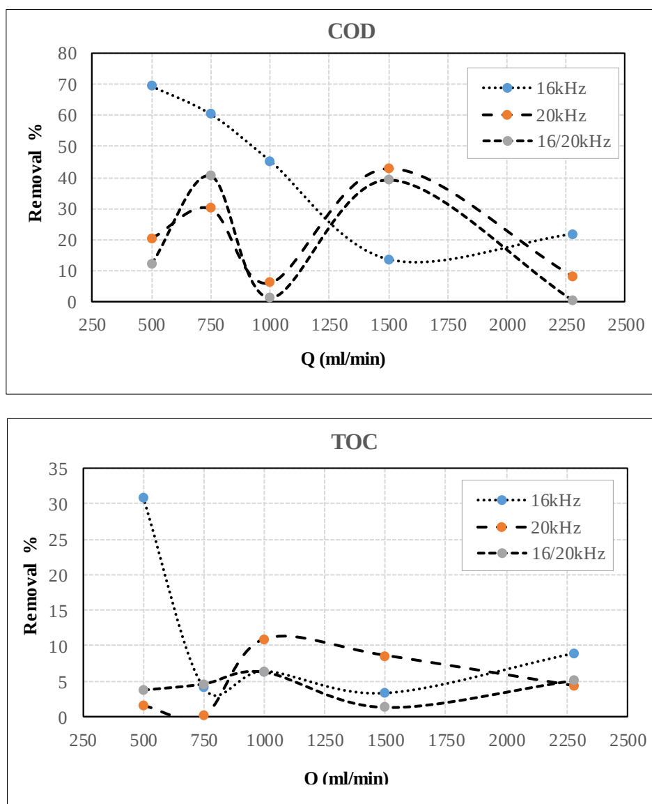
Figure 3. High-strength wastewater sonication in the flow-through ultrasound reactor
