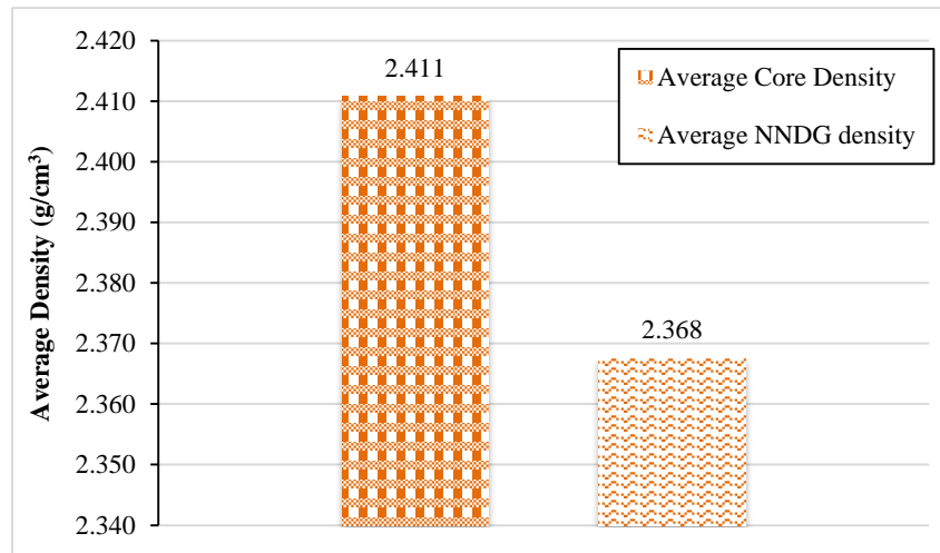
Figure 10. Average density data for site 1; Sahiyan wala interchange (Faisalabad Multan motorway)
