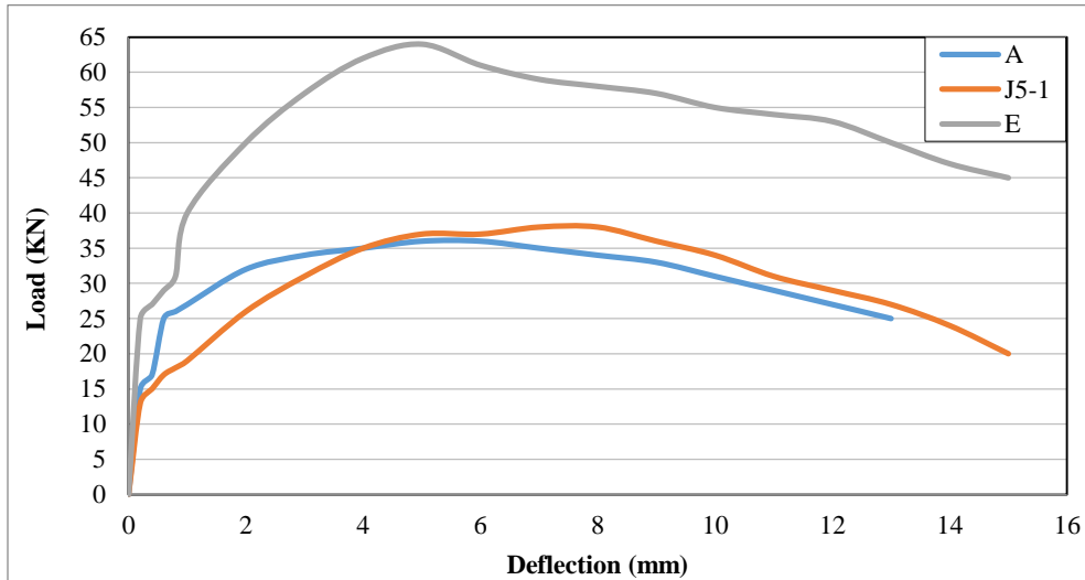
Figure 6. Load-deflection curve at mid-span for Concrete beams strengthened with 5 cm of Jute Fibers compared with reference beams and Carbon Fibers beams
